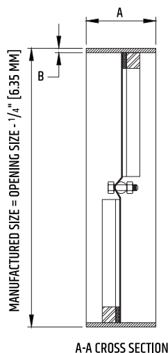
A-A CROSS SECTION
