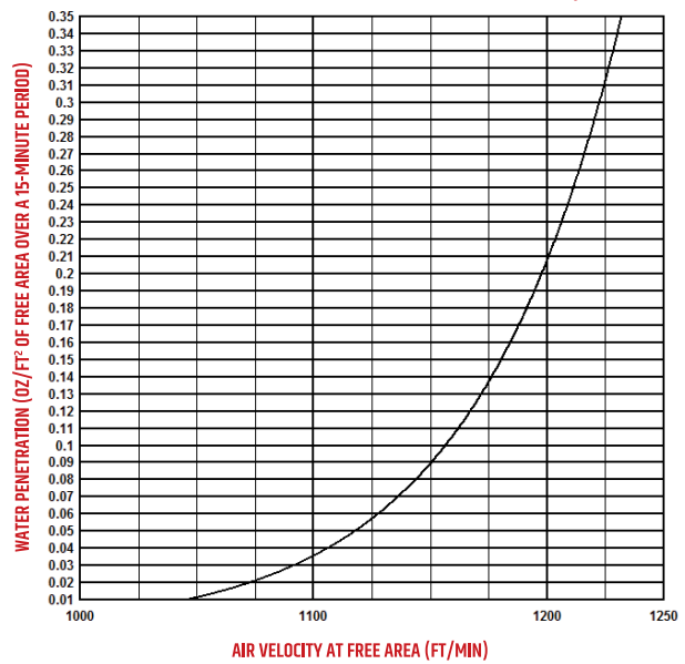
WATER PENETRATION MODEL TWGW-646 BEGINNING POINT OF WATER PENETRATION AT 1 045 FT/MIN
