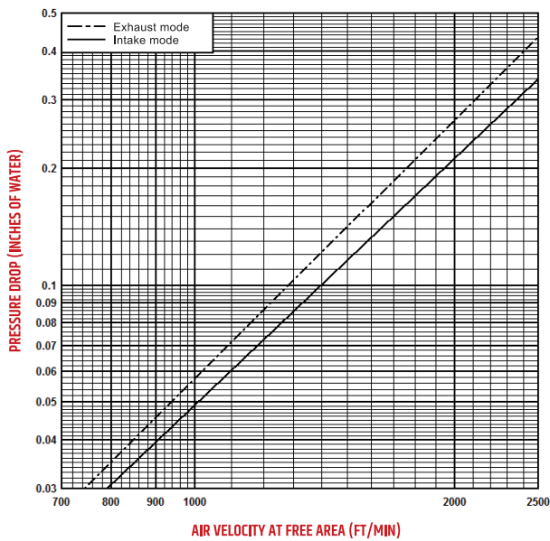
PRESSURE DROP VS AIR VELOCITY MODEL TWGW-646
